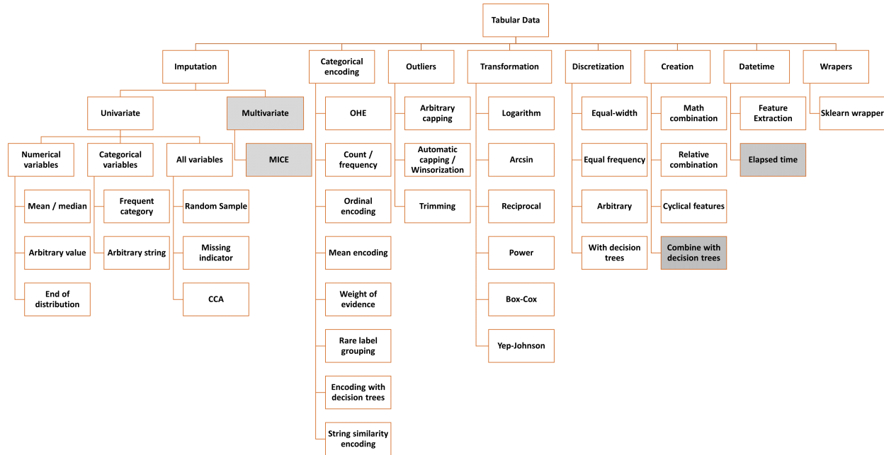
Fig. 12: Transformers for tabular data
