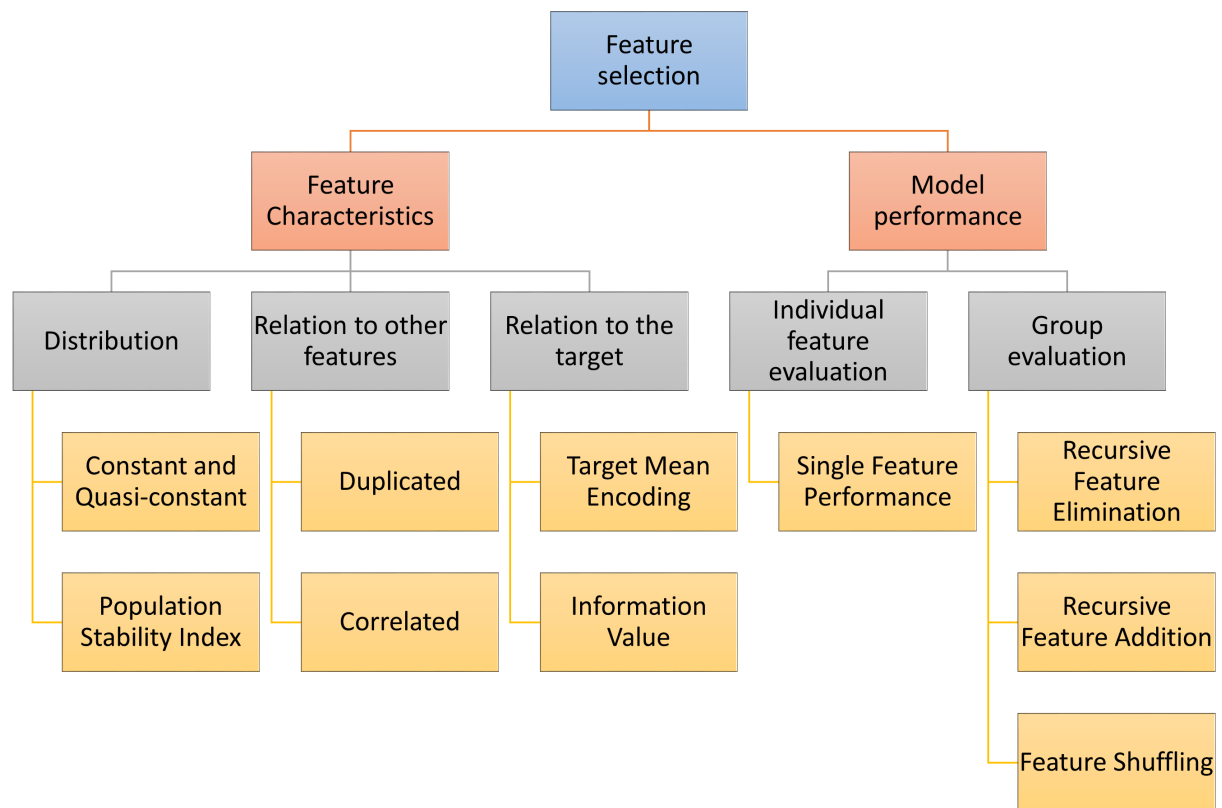
Fig. 2: Selection mechanisms - Overview
