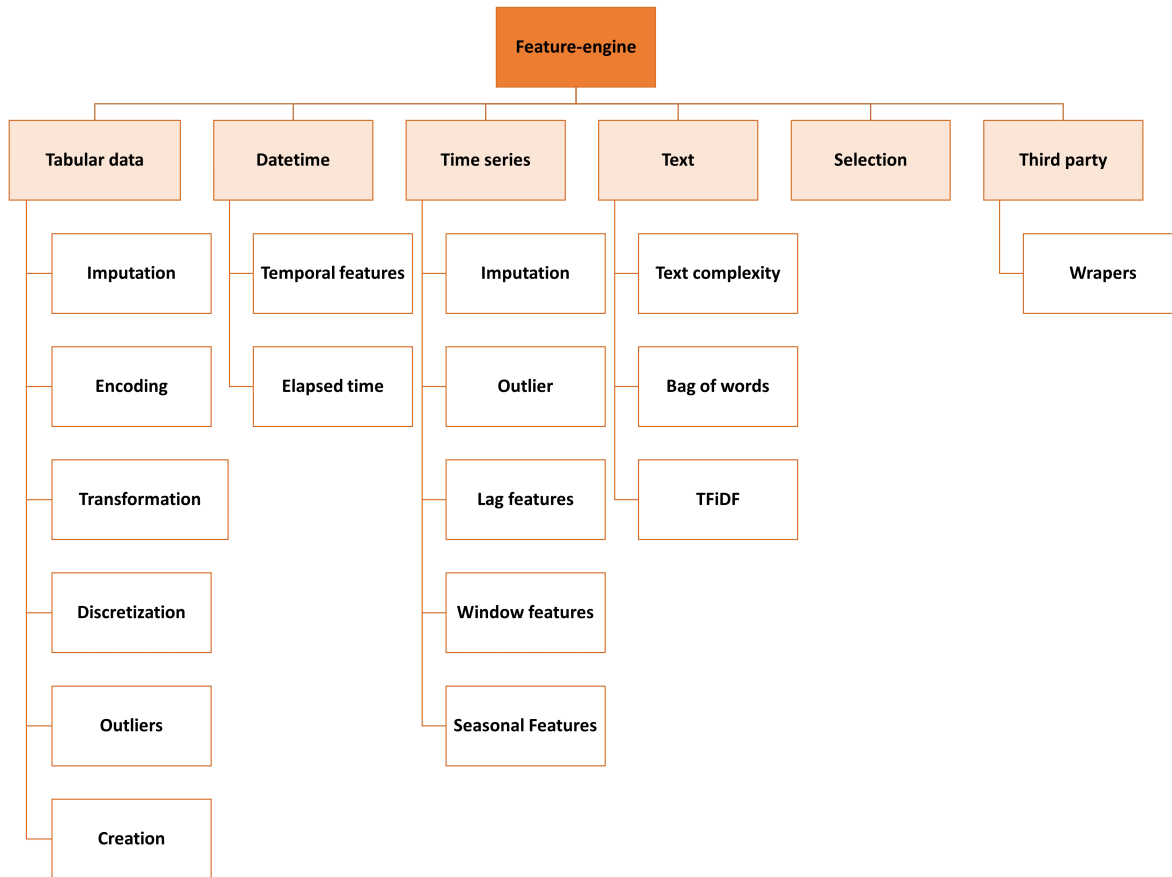
Fig. 11: Feature-engine structure
